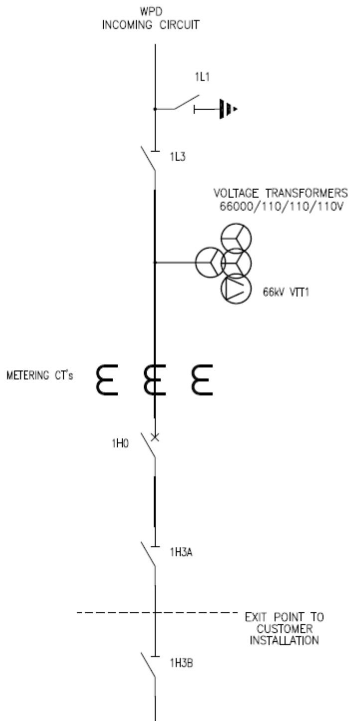
SINGLE CIRCUIT TEED CONNECTION
