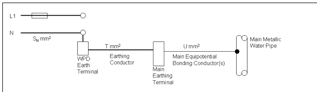
Figure 22 – TN-C-S (PME) Bonding Requirements
