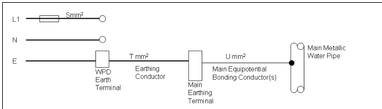
Figure 24 – TN-S (SNE) Bonding Requirements
