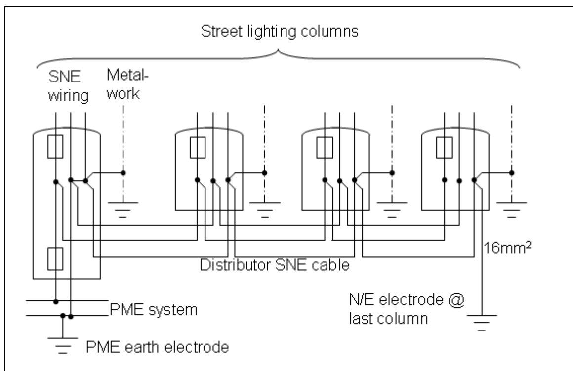
Figure 7 –SNE Distributor Fed from PME Service
