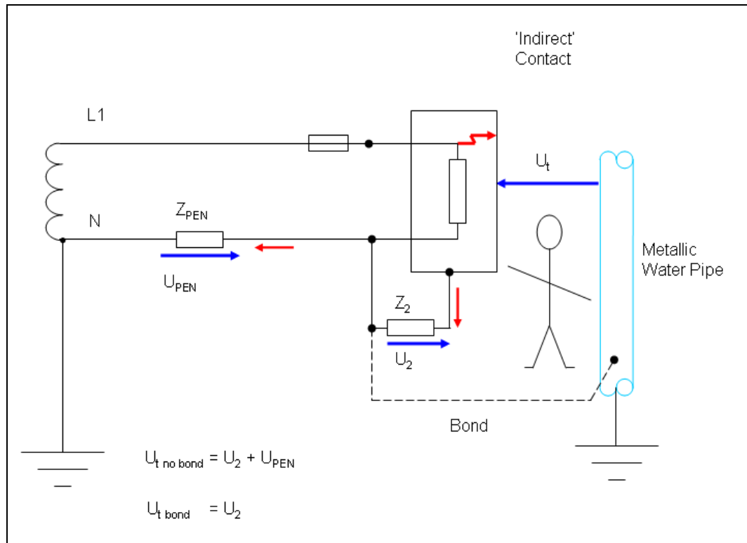
Figure 16 – Effect of Bonding on Indirect Contact Touch Voltage
