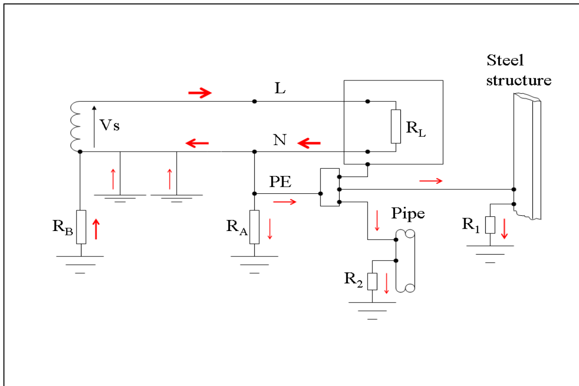
Figure 21 – Neutral Current Diversion with PME
