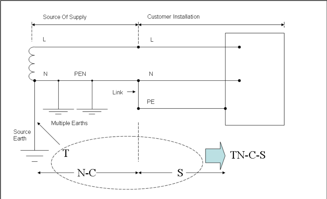
Figure 10 – TN-C-S Type of Earthing
