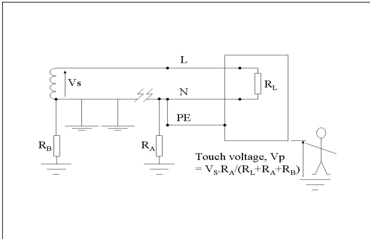
Figure 19 – Touch Voltage Control By Earth Electrode Beyond PME Neutral Break
