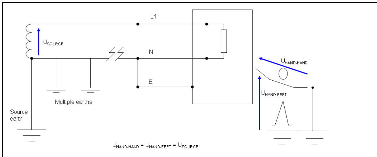
Figure 18 - Touch Voltage For Broken Neutral – TN-C-S (PME) System
