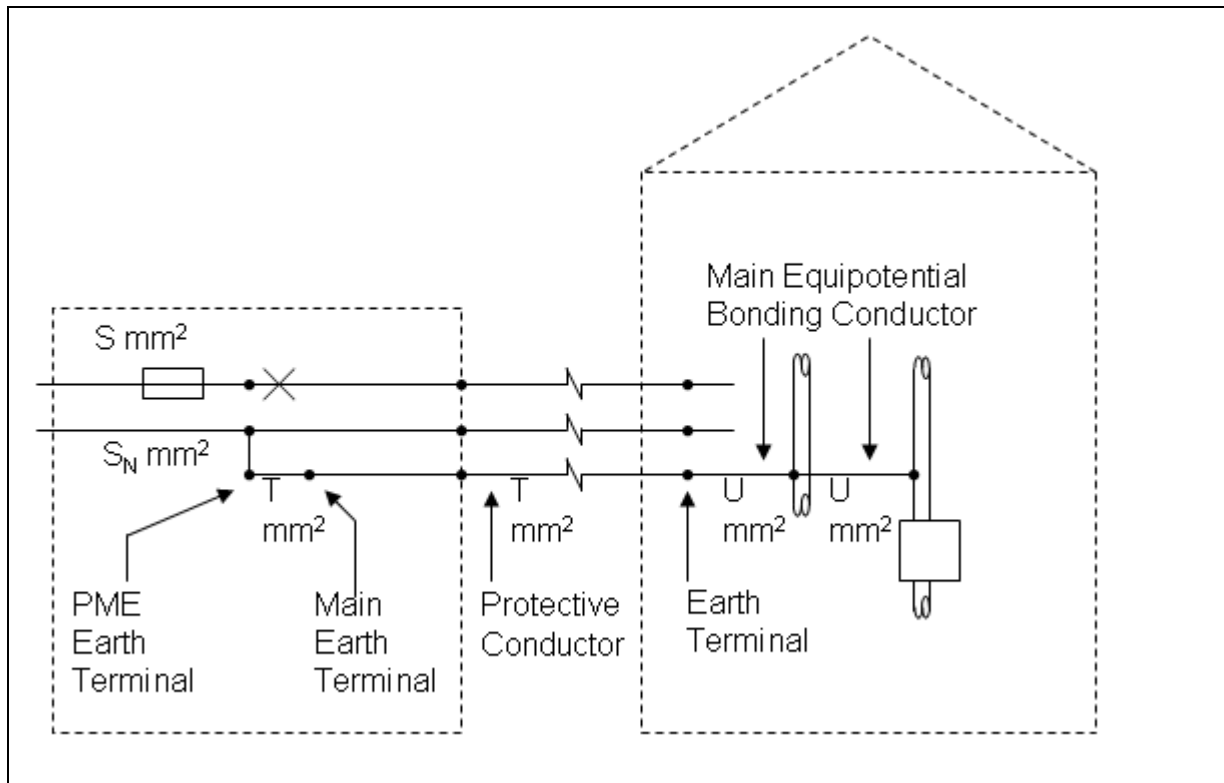
Figure 23 – Bonding Requirement - Service Terminating In A Separate Building
