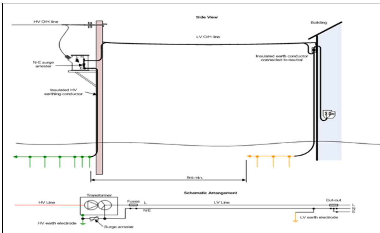
Figure 13 – PNB variant – TN-C-S
