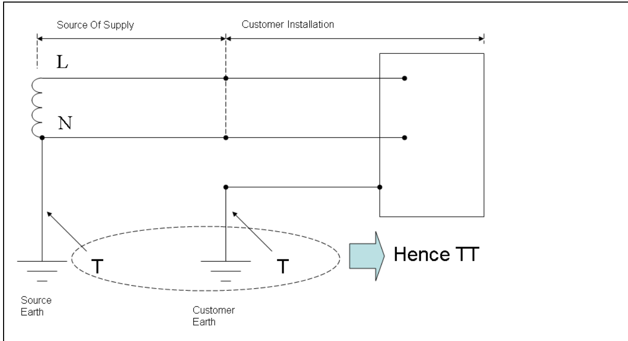
Figure 11 – TT Type of Earthing
