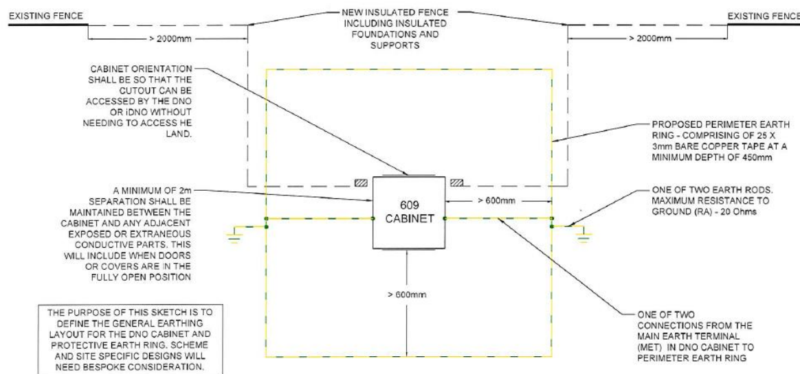
Figure 8 - Metallic Pillar Earthing Arrangements At Highways England Sites
