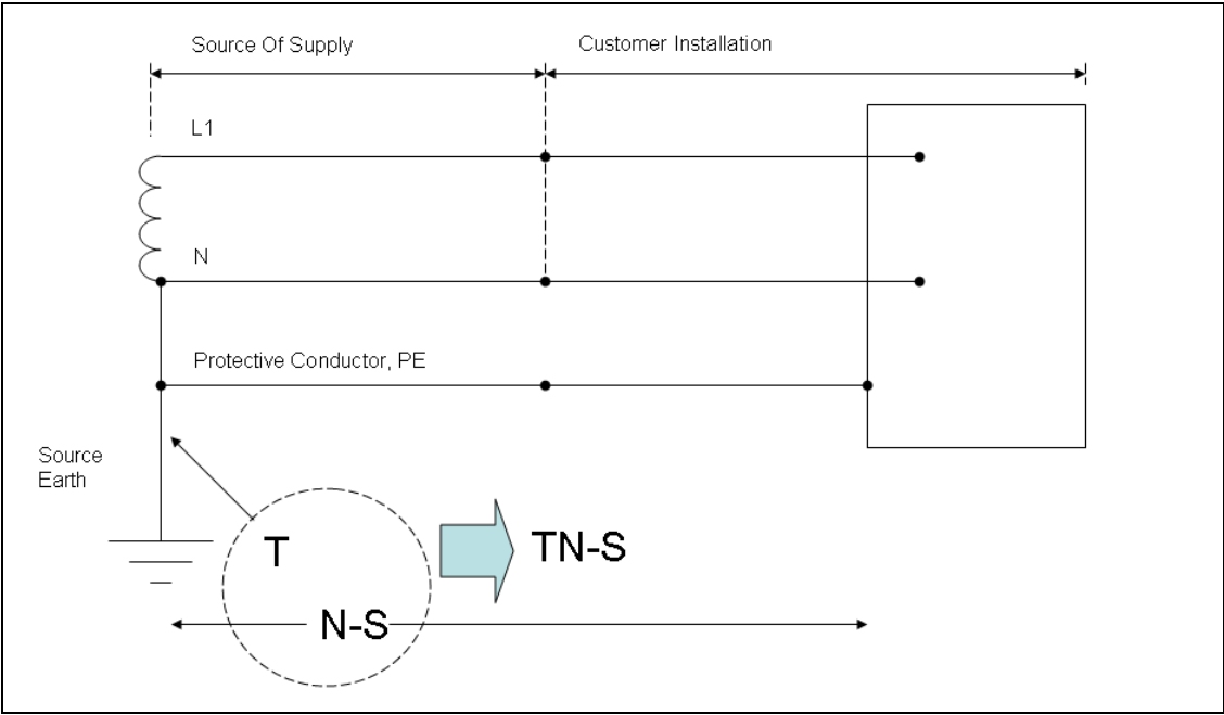
Figure 9 – TN-S Type of Earthing
