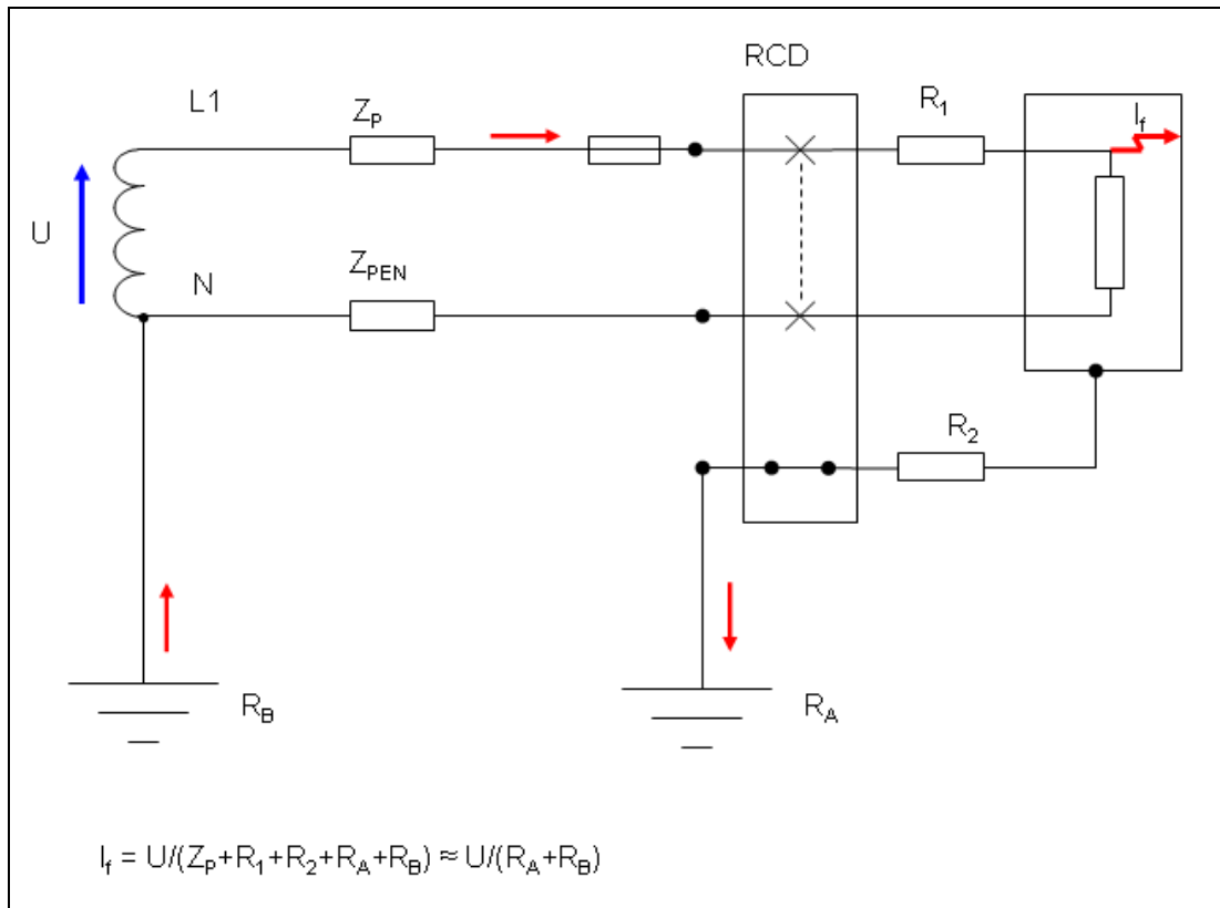
Figure 17 – RCD Protection for TT System
