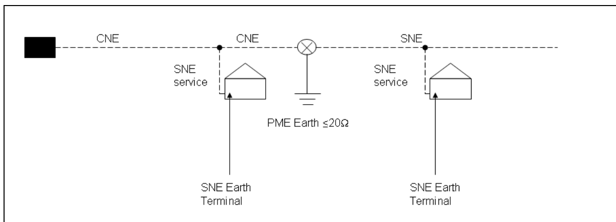
Figure 3 - 20Ω Rule
