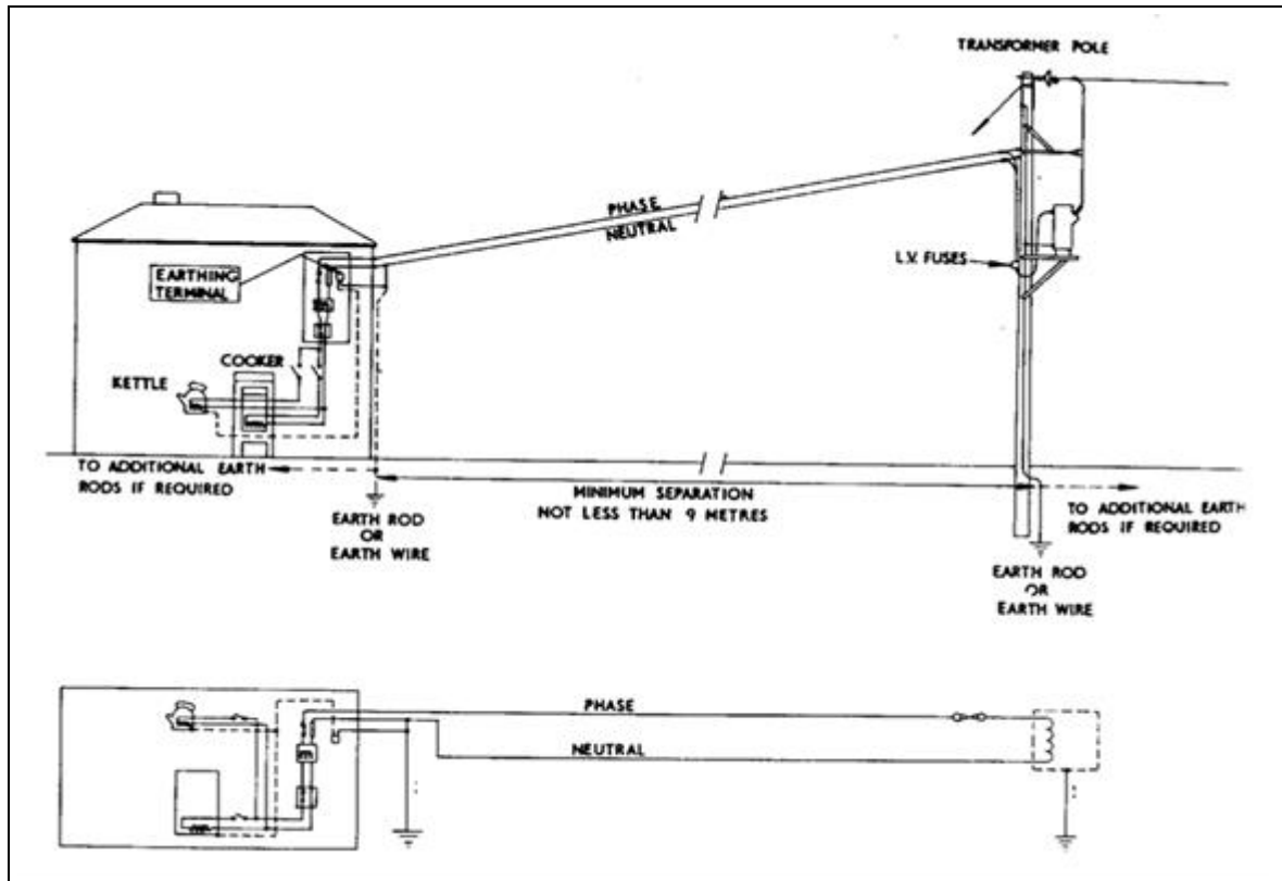
Figure 12 – PNB variant with aerial overhead service – TN-S
