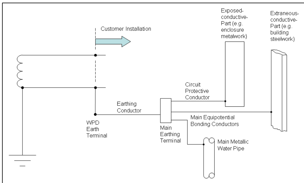
Figure 15 – Earthing Terminology – Customer's Installation
