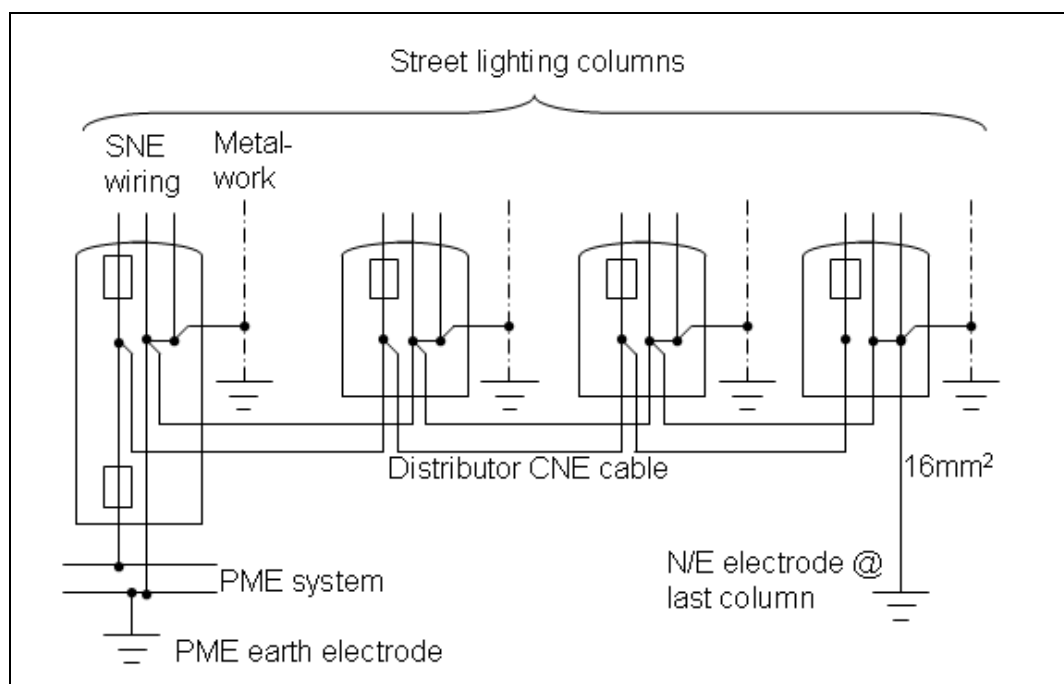
Figure 6 CNE Distributor Fed from A PME Service
