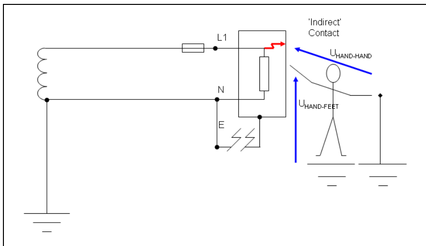
Figure 14 – Indirect Contact Electric Shock Hazard – Metalwork Uneearthed
