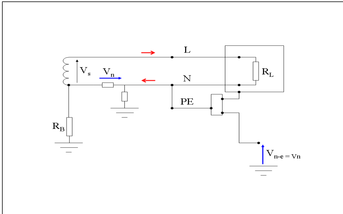
Figure 20 – Neutral-Earth Voltage on PME Earth Terminal
